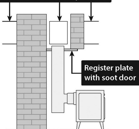
Alternative soot door positions
